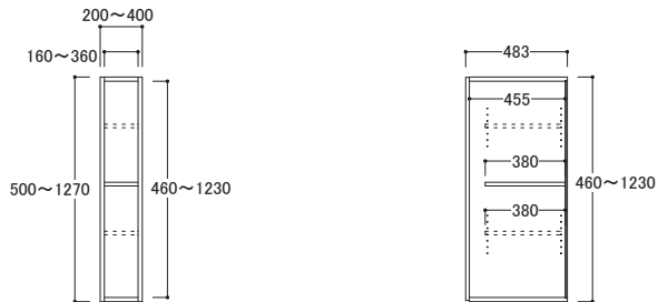
IK/IU-□SBUL/□SBUR ● 外寸 W200~400xD483xH500~1270mm ● 共通側面図
