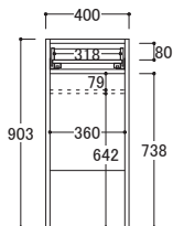
IK/IU-□40B2 ● 外寸 W400×D433×H903mm 取手含むD455mm)
