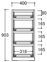
IK/IU-□40DH2 ● 外寸 W400×D433×H903mm 取手含むD455mm)
