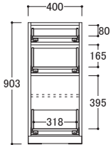
IK/IU-□40D2 ● 外寸 W400×D433×H903mm 取手含むD455mm)
