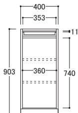
IK/IU-□40CKL2/40CKR2 ● 外寸 W400×D433×H903mm 取手含むD455mm)
