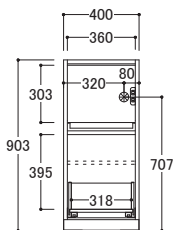
IK/IU-□40G2 ● 外寸 W400×D433×H903mm 取手含むD455mm)
